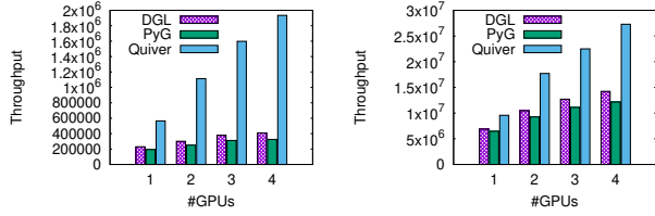
(a) ogbn-products (b) ogbn-papers100M Fig. 11: Scalability with single multi-GPU server
