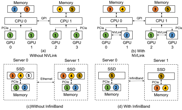
Fig. 8: Feature placement scenarios
