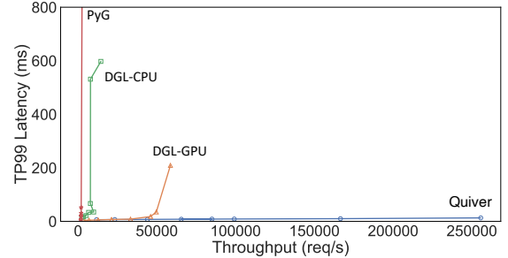
Fig. 9: Throughput vs. latency of GNN request serving
