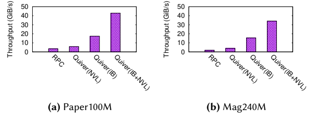
Fig. 16: Throughput of feature collection
